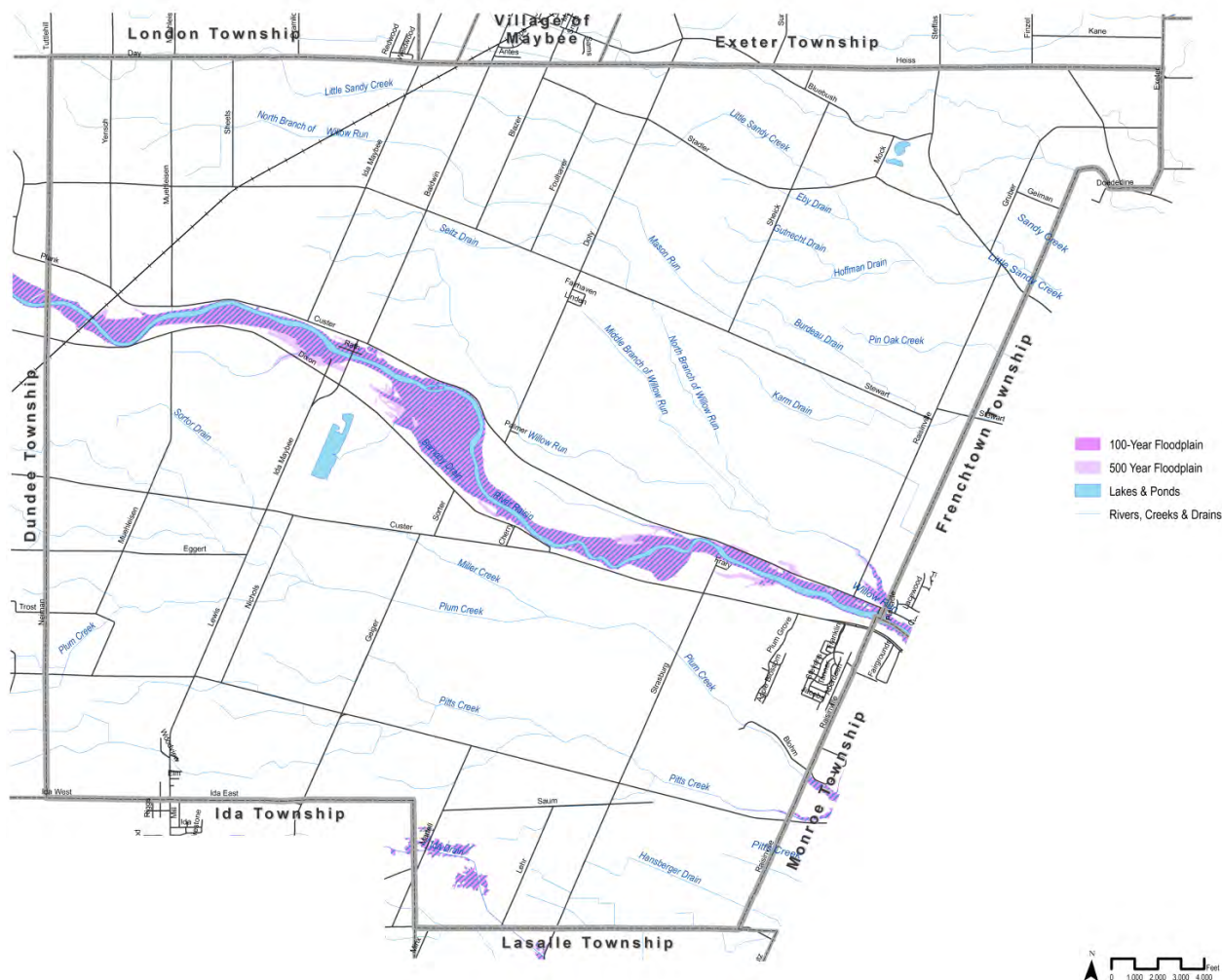
Figure 11. Surface Hydrology
