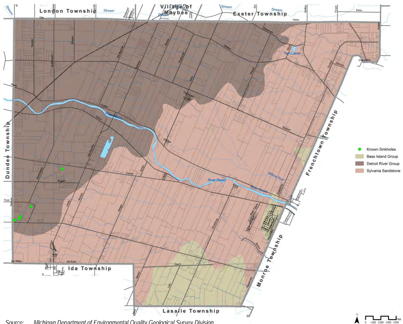
Figure 8. Bedrock Geology
