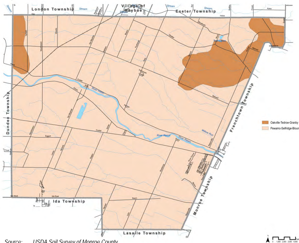
Figure 9. Soil Associations
